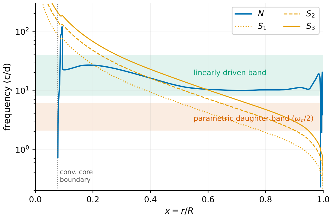
Propagation diagram, M = 1.85 M_{\odot} \delta Sct model
